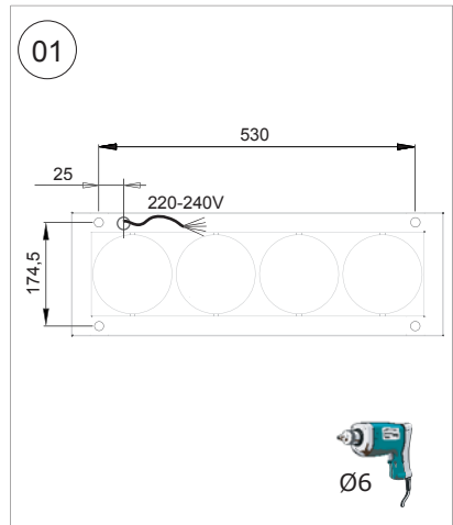
HOLE PATTERN
