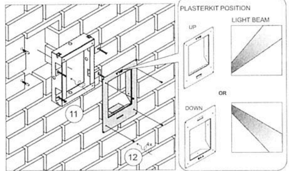
MOUNTING SEQUENCE FOLLOW Nr. 11-15
