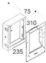
CONCRETE BOX 139 276 04 98
