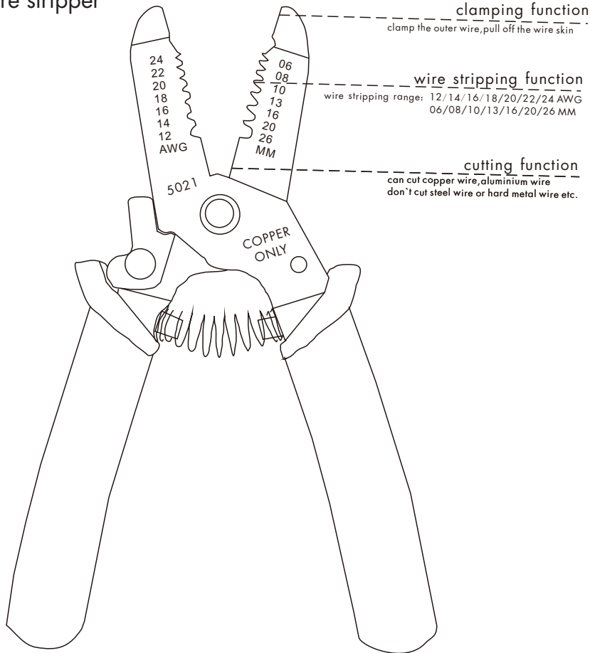
Wire stripper
